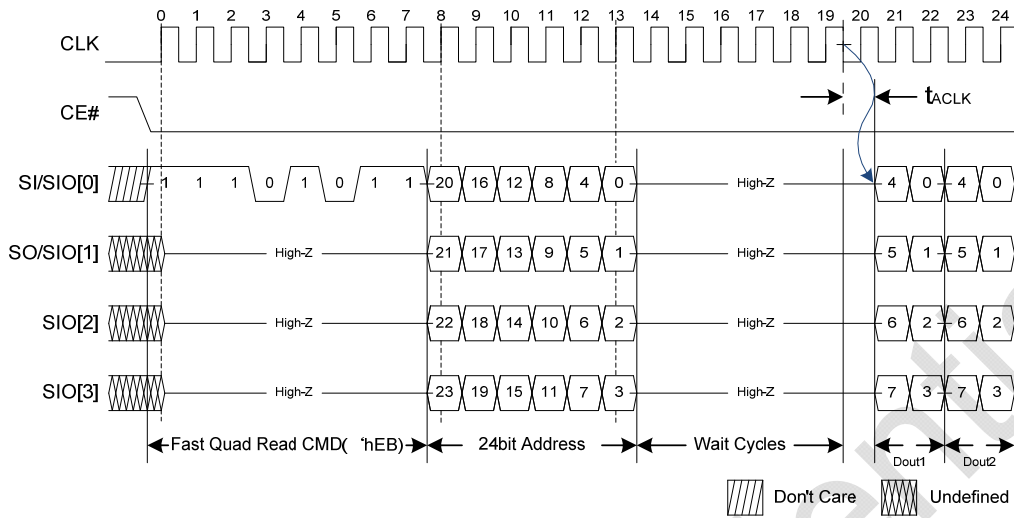
Figure 8 : SPI Fast Quad Read 'hEB' (MAX. freq. 133MHz)
