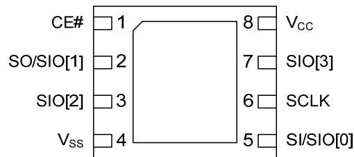
WSON(See Through with Top View)
